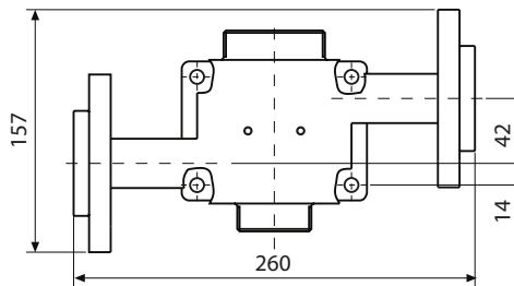
DN 25 flange, 180° staggered with connection for cleaning system
